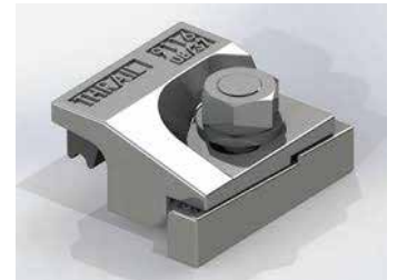
CRANE RAIL CLIPS
